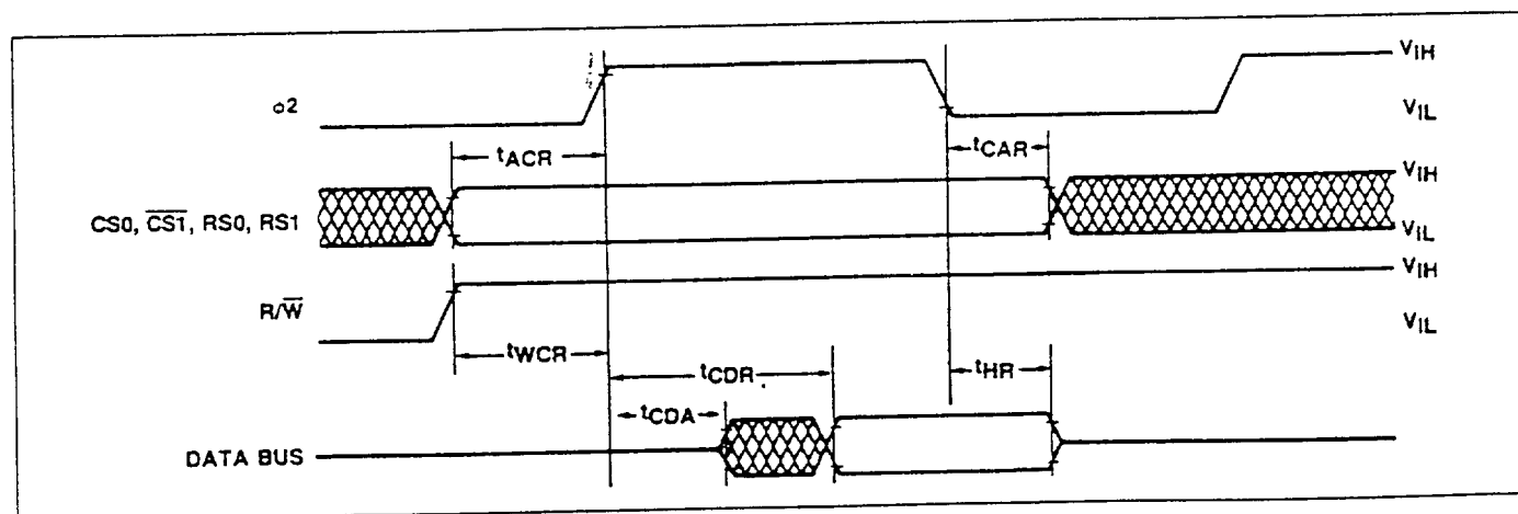
Read Timing Diagram
