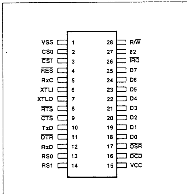
Figure 1. R6551 ACIA Pin Configuration
