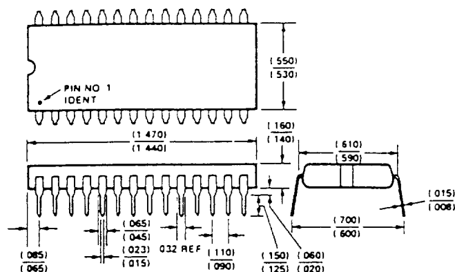
28-PIN PLASTIC DIP
