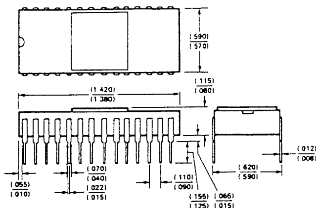
28-PIN CERAMIC DIP
