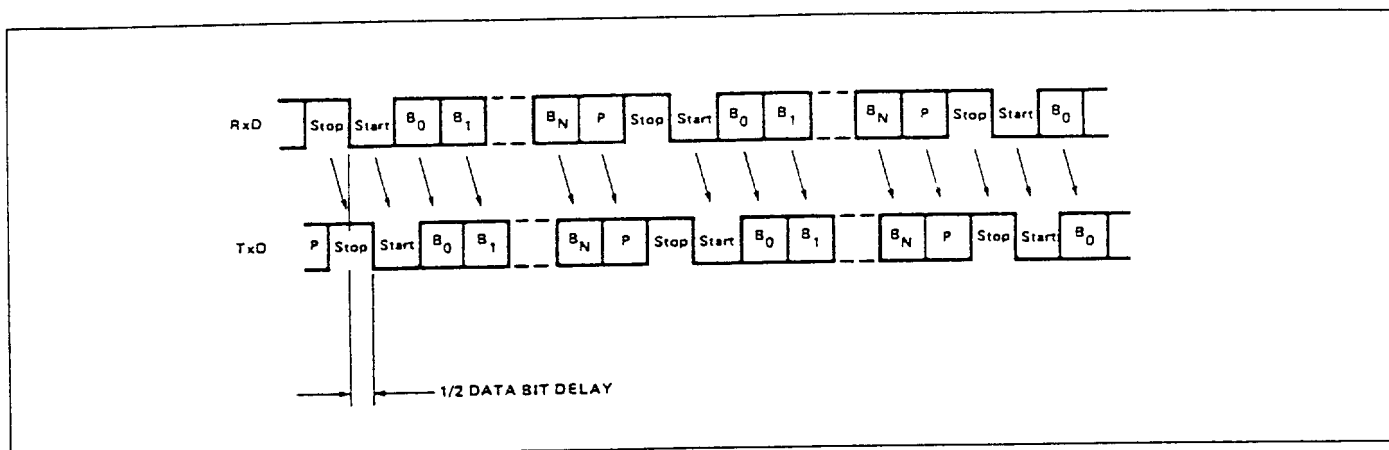
Figure 10. Echo Mode Timing
